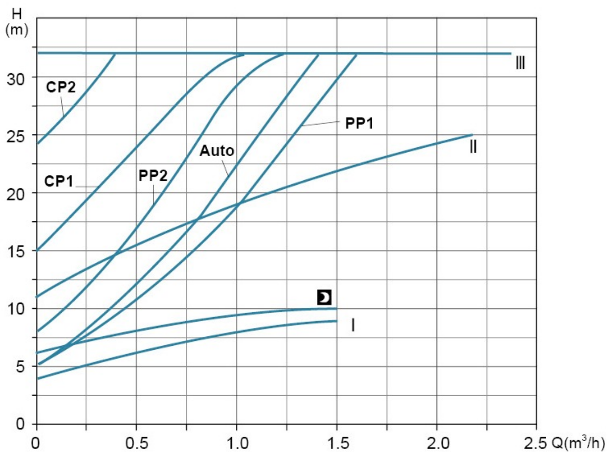
ARPXX-50 Q-H
