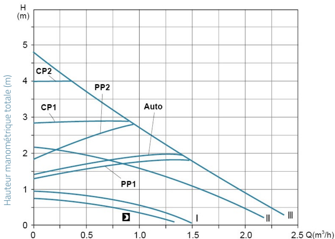
ARPXX-50 Q-H
