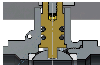
O-ring
